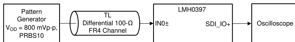
Figure 23. Test Setup for LMH0397 in CD Mode
