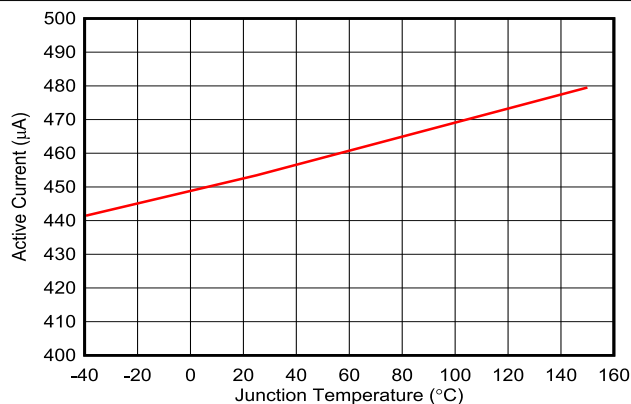
图 6-4. V_{IN} Active Current Versus Temperature
