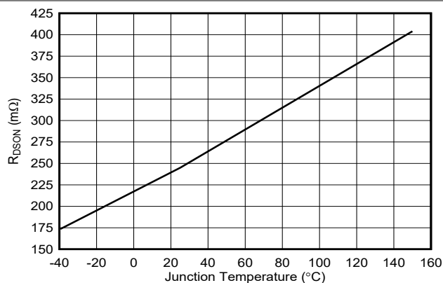
图 6-6. MOSFETs On-State Resistance Versus Temperature
