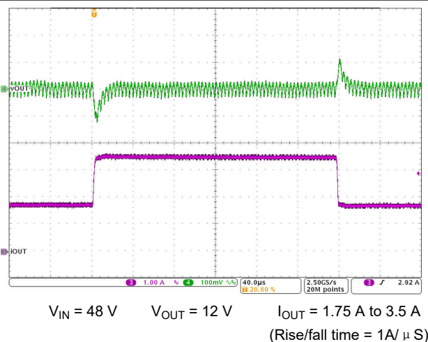
图 8-5. Load Step Response
