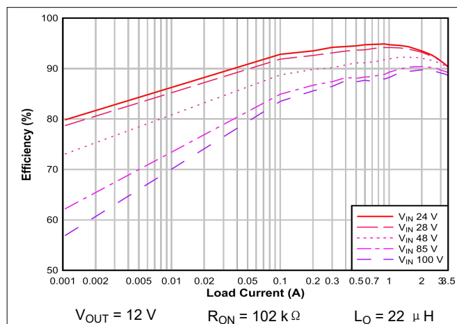
图 8-2. Conversion Efficiency (Log Scale)
