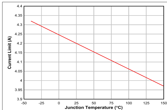
图 6-7. Peak Current Limit Versus Temperature
