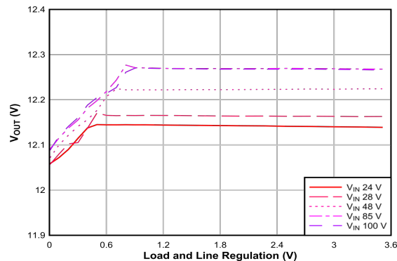
图 6-2. Load and Line Regulation
