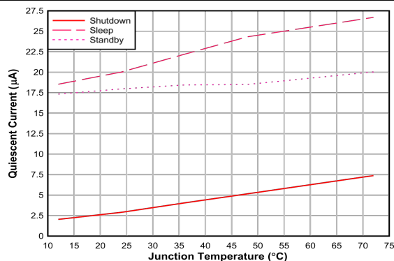
图 6-3. Shutdown, Sleep, and Supply Current Versus Temperature
