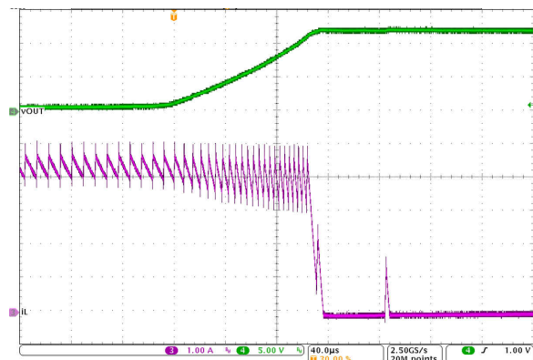
图 8-8. Short Circuit Recovery
