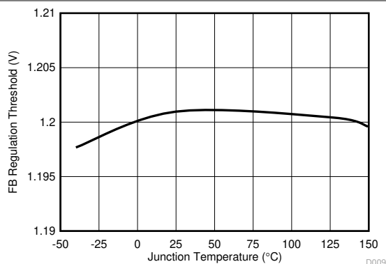
图 6-5. Feedback Comparator Threshold Versus Temperature
