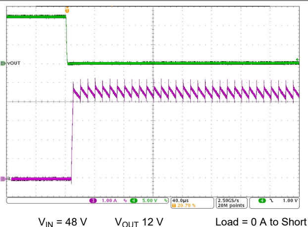
图 8-7. Short Circuit Applied
