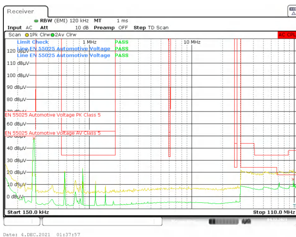
图 8-10. Full-Load Switching
