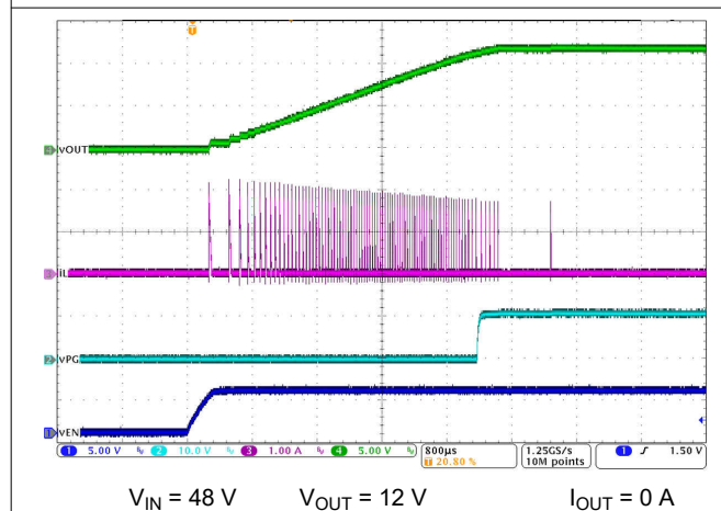
图 8-6. No-Load Start-Up with EN/UVLO
