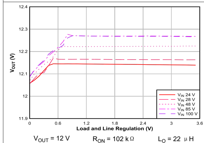
图 8-4. Load and Line Regulation Performance
