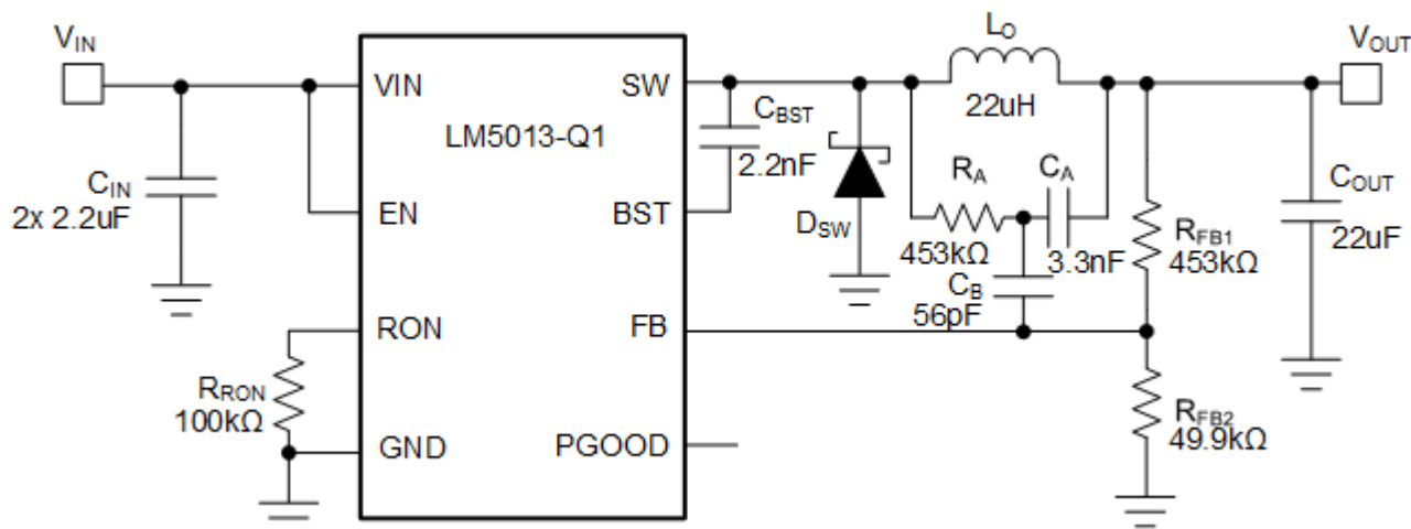
图 8-1. Typical Application, V_{IN(nom)} = 48\text{ V} , V_{OUT} = 12\text{ V} , I_{OUT(max)} = 3.5\text{ A} , F_{SW(nom)} = 300\text{ kHz}
