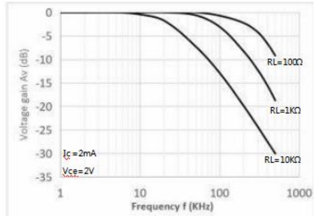
Fig.8 Frequency Response
