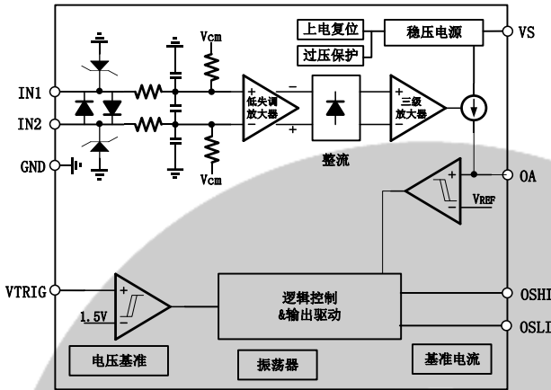
Figure 6. SS4129 Block Diagram
