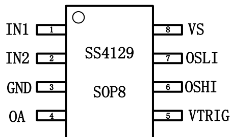
Figure 5. Pin Configuration
