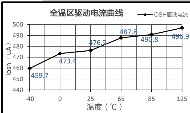
Figure 3. I OSH Curve In -40°C~125°C
