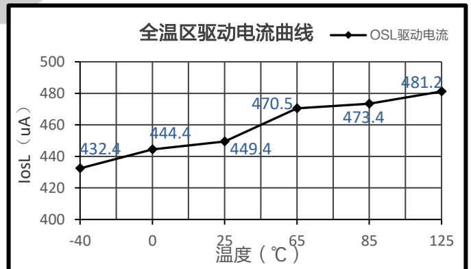
Figure 4. I OSL Curve In -40°C~125°C
