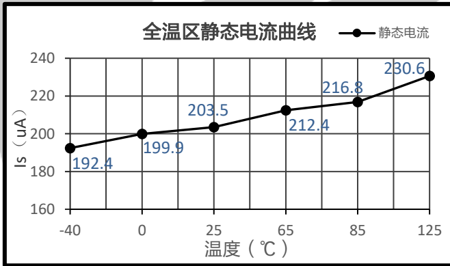
Figure 2. I S Curve In -40°C~125°C
