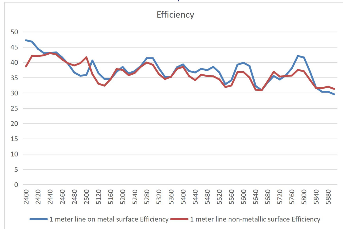
Efficiency (%)
