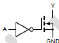
Figure 3. Logic diagram
