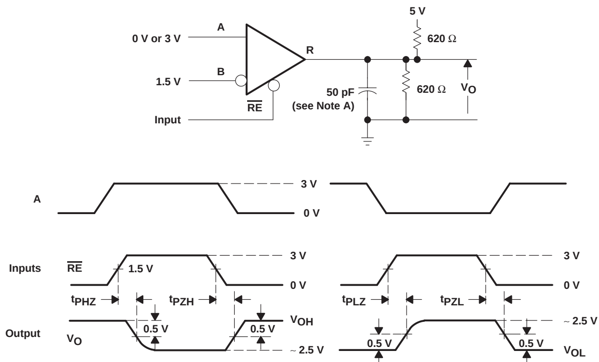
Figure 8. Receiver t_{PZH} , t_{PHZ} , t_{PLZ} , and t_{PZL} Test Circuit and Voltage Waveforms
