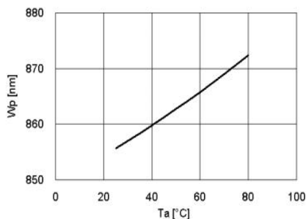
Fig.5 – Peak Wavelength (@50mA) vs. Ambient Temperature
