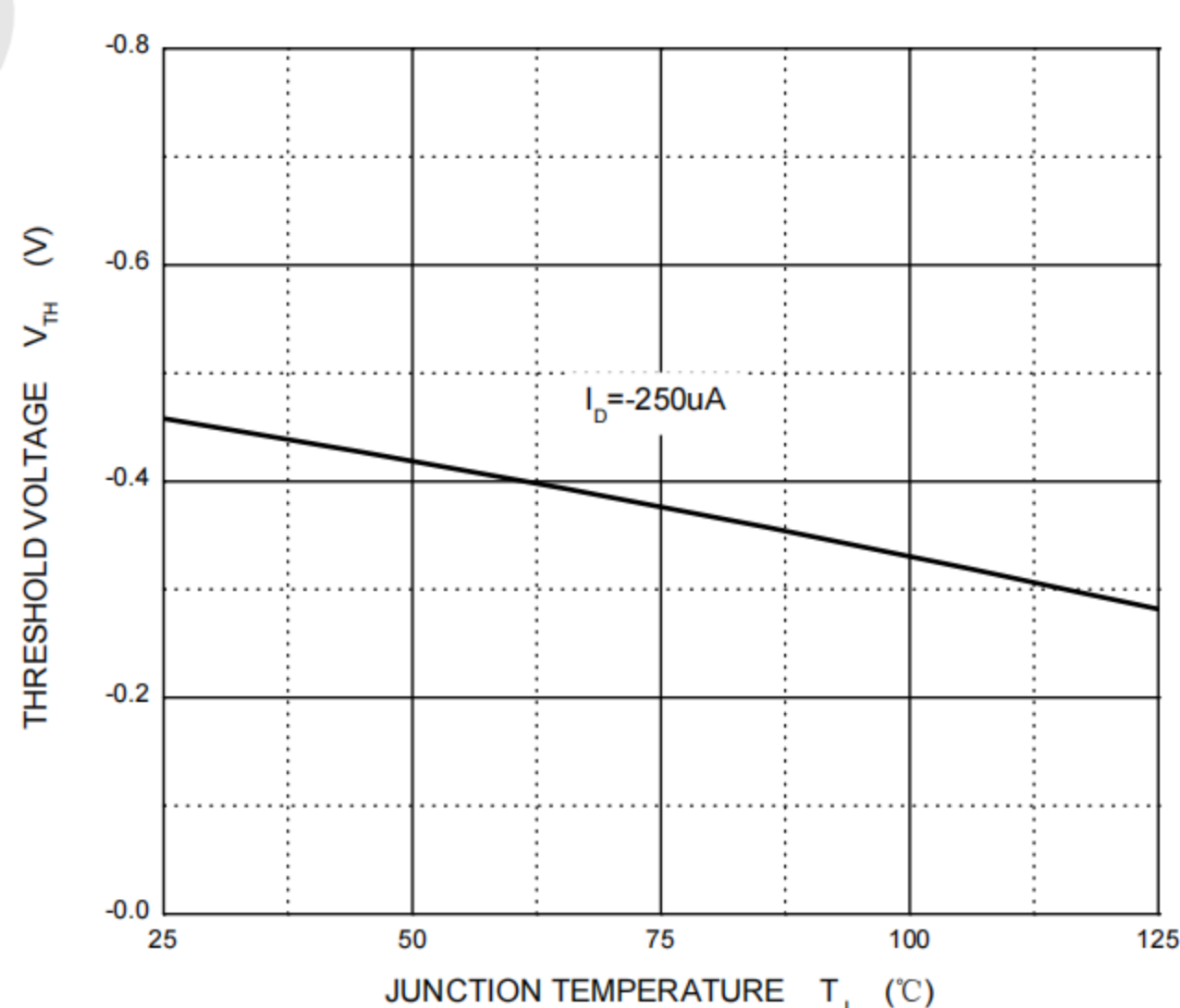
Threshold Voltage
