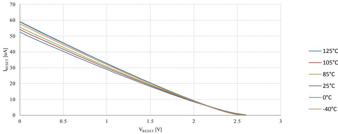
Figure 23-35. Reset Pull-up Resistor Current vs. Reset Pin Voltage ( V_{CC} = 5V )
