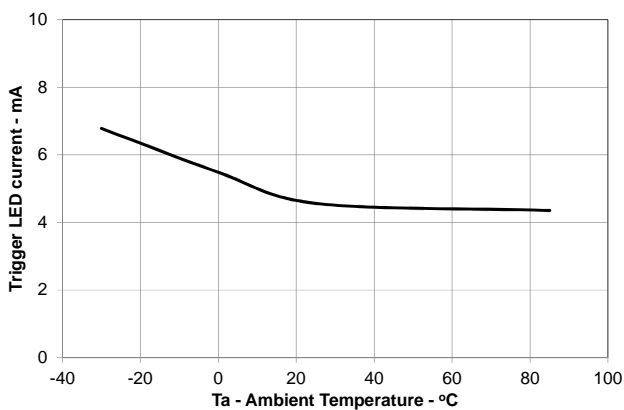
Fig 3. Trigger LED current vs. Ambient Temperature
