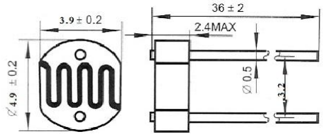
Dimensions in millimetres
