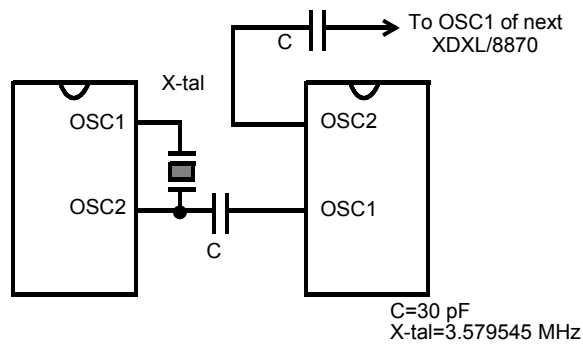
Figure 7 - Oscillator Connection
