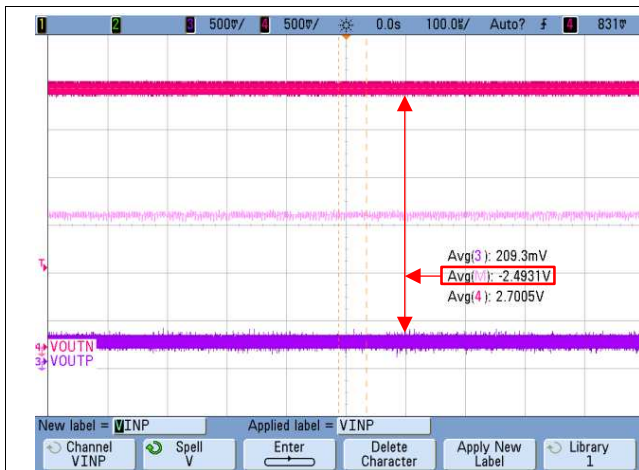
Figure 47. Typical Negative Clipping Output of the AMC1301
