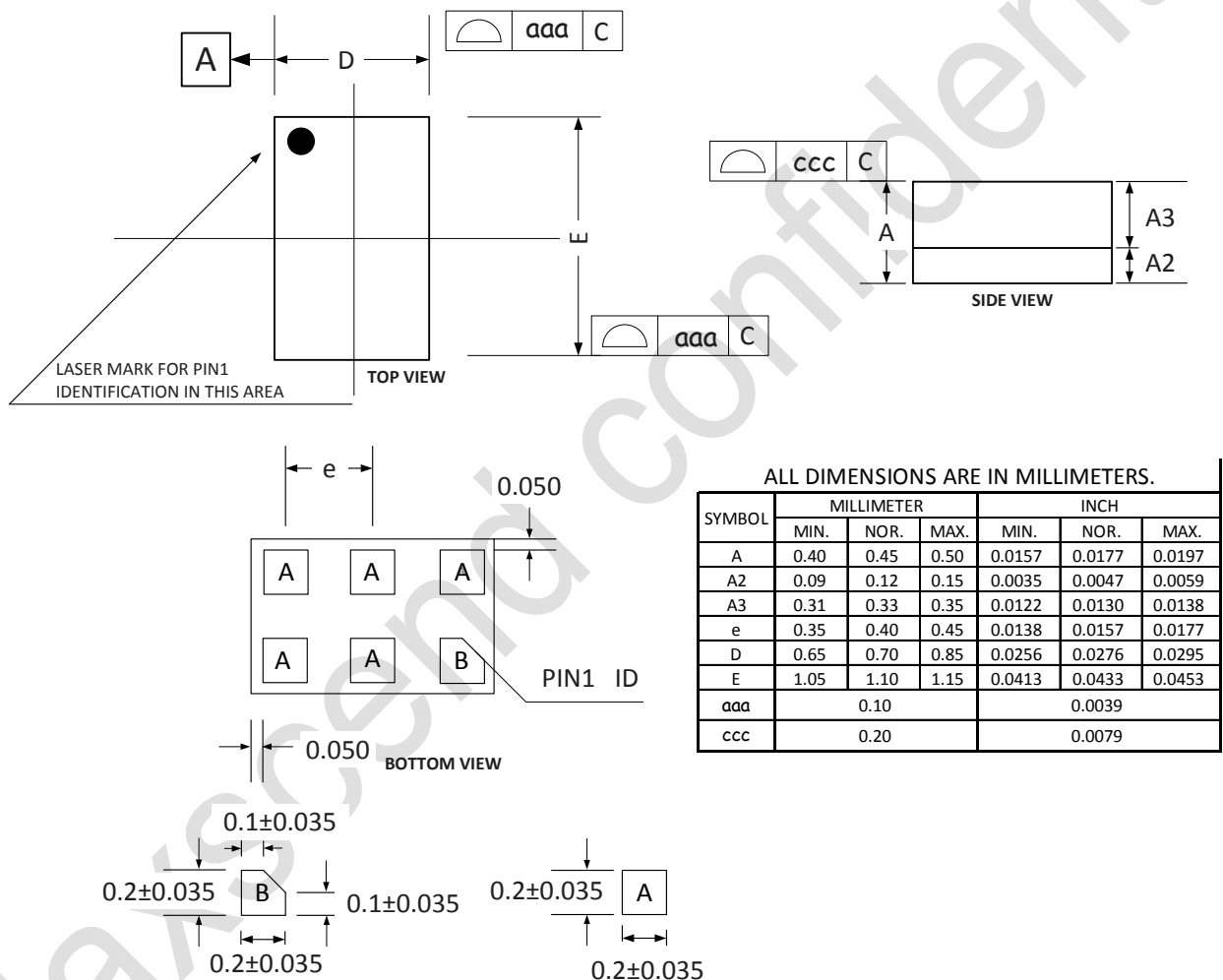
Figure 2. MXDLN16T outline dimension
